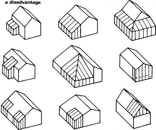
6 Alternative ways of adding glass structures to existing buildings
